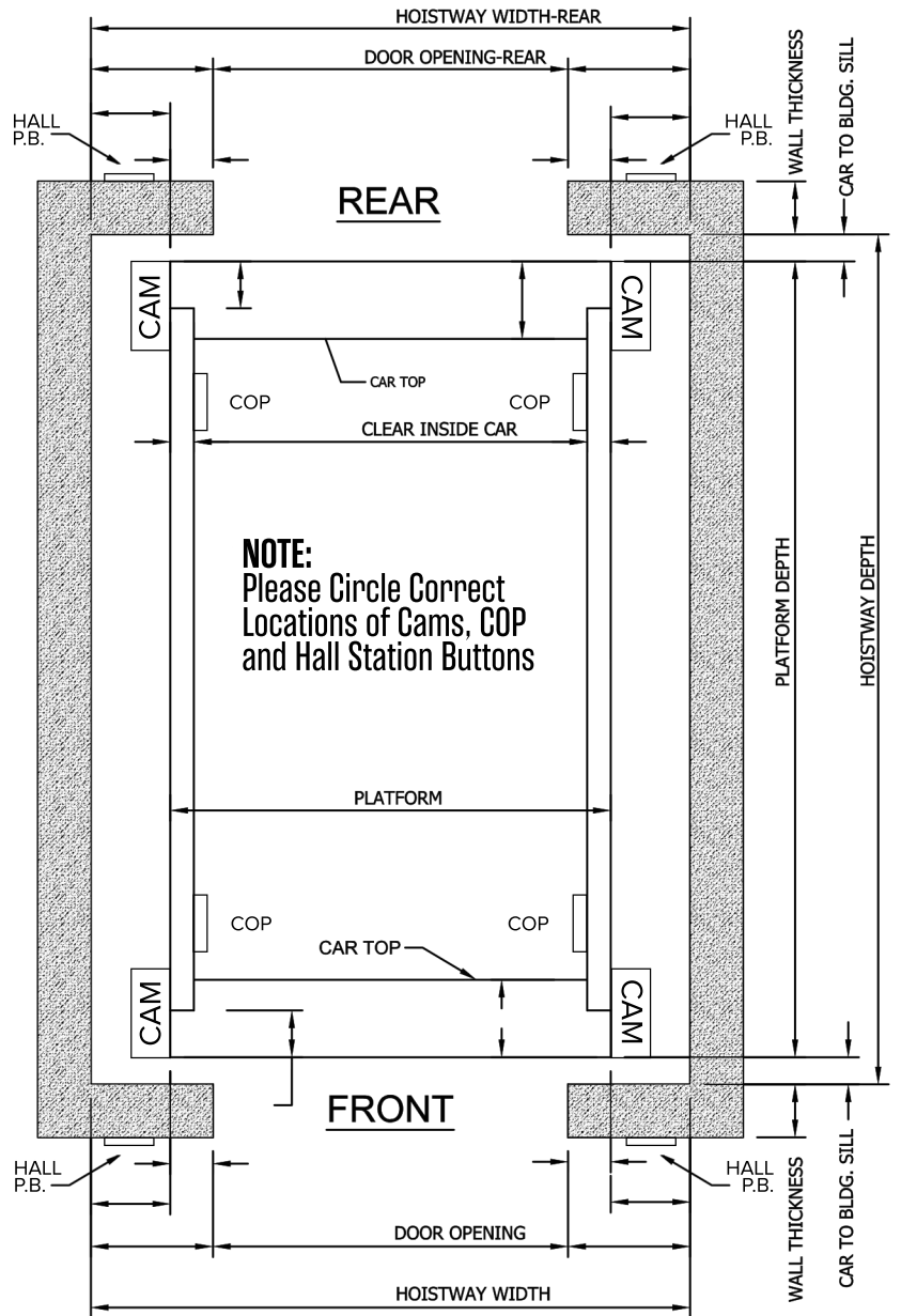
PLAN
